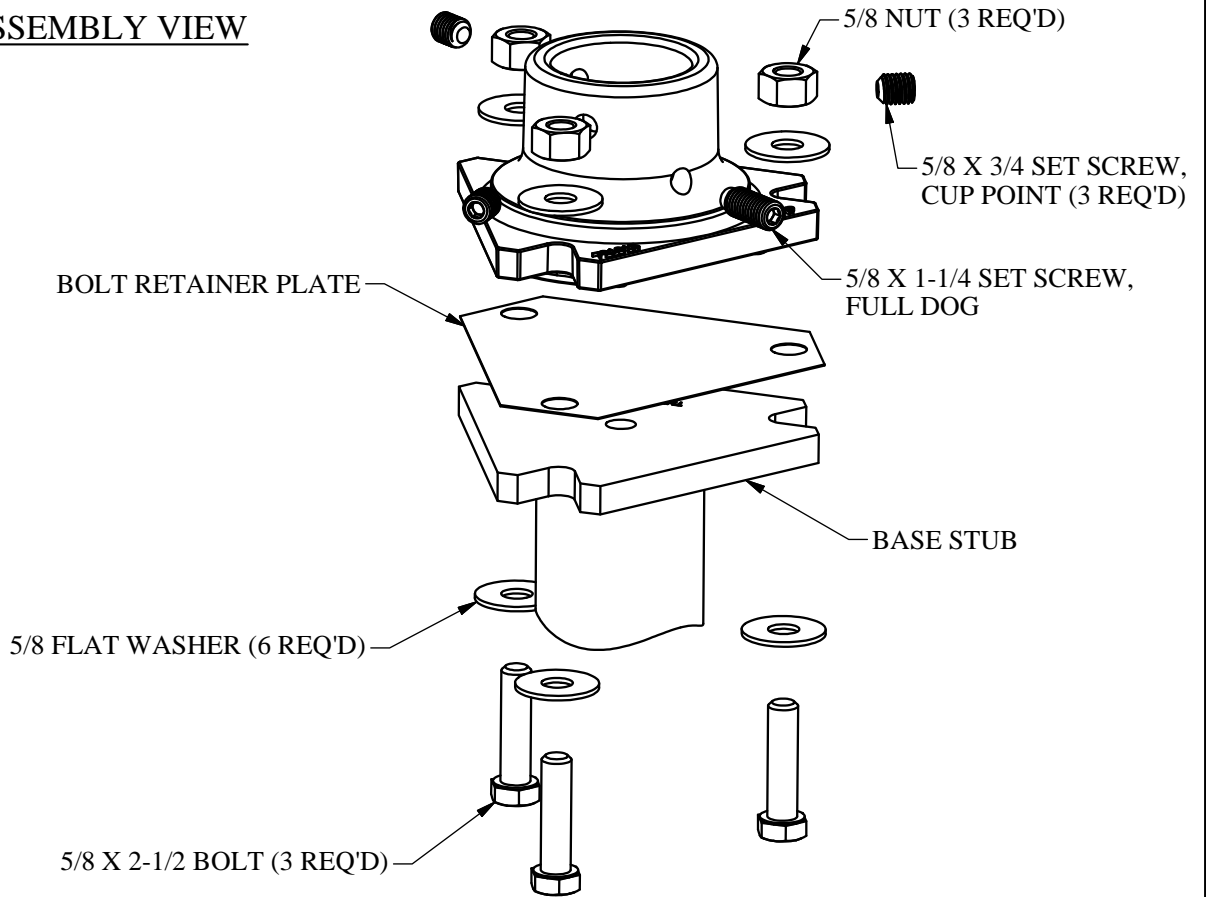
EXPLODED VIEW
