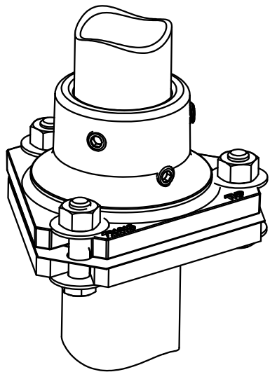
ASSEMBLY VIEW
